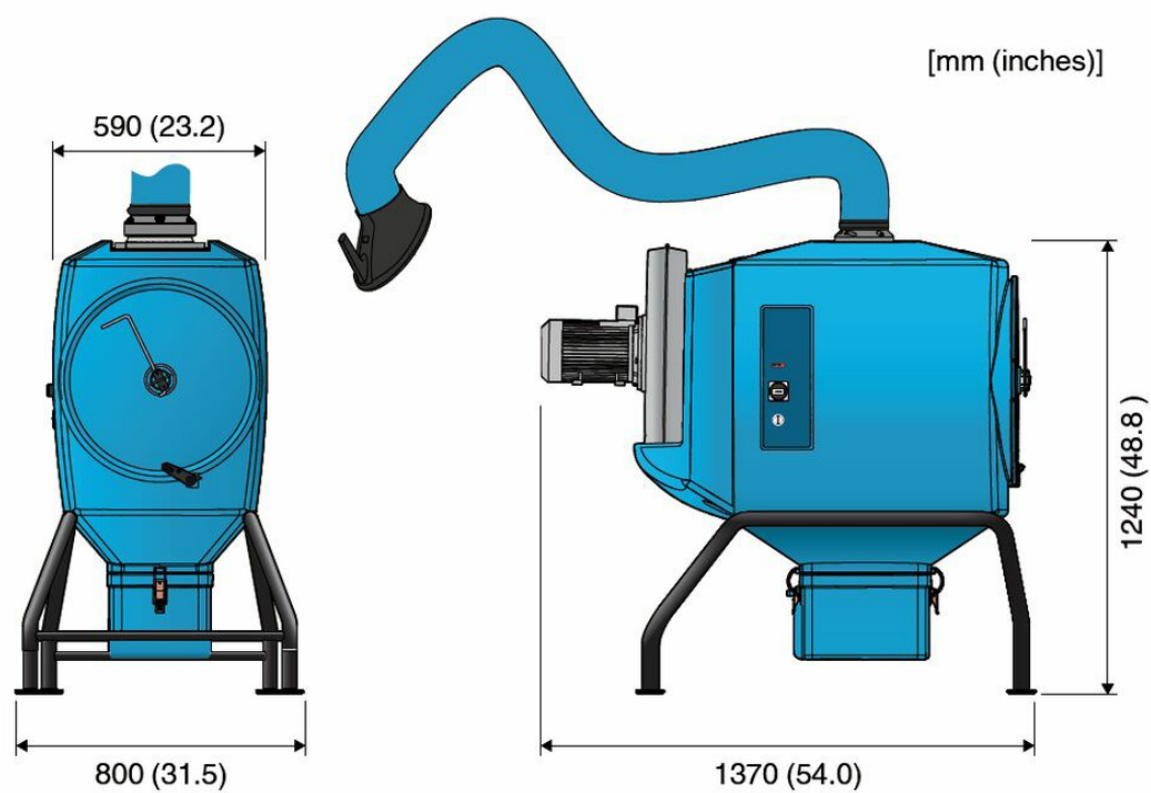
Floor mounted FilterBox 12M
