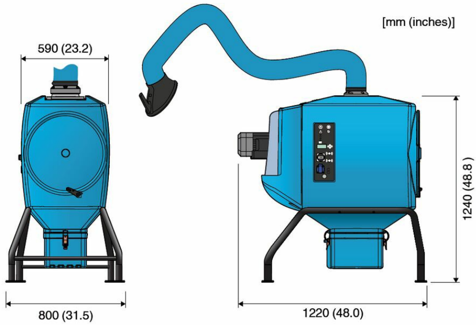
Floor mounted FilterBox 10A
