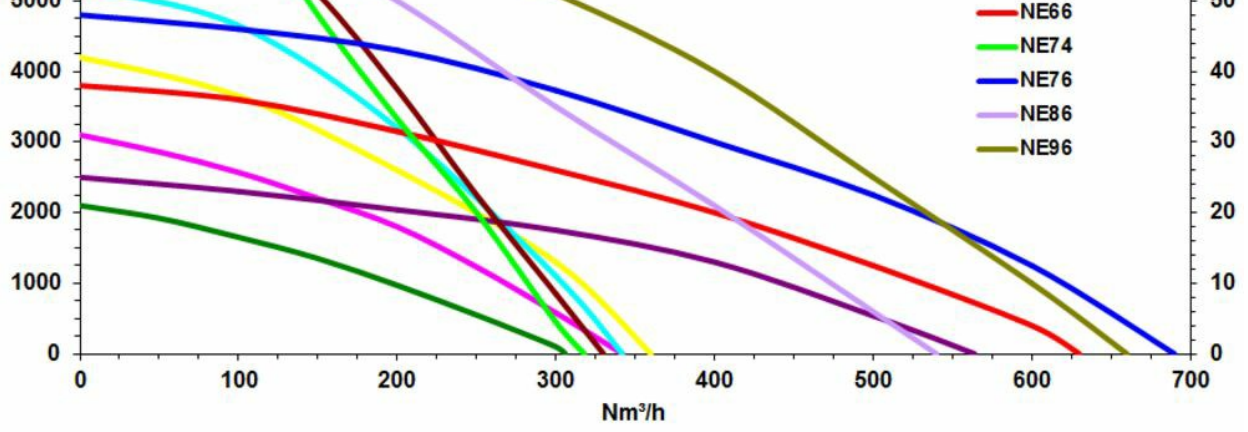
Air Powered ejectors All performance data are based on 7 bar supply pressure
