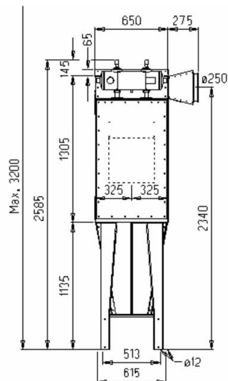
FMK(Z)25-2E Flange All dimensions in mm. * 65 mm to be included at top mounted fan.
