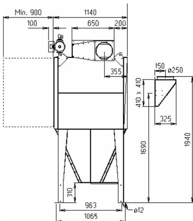
FMK(Z)25-2E Flange All dimensions in mm. * 65 mm to be included at top mounted fan.
