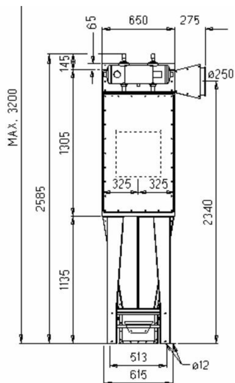
FMK(Z)25-2E Bin All dimensions in mm. If 50 liter bin with rollers, add 90 mm. * 65 mm to be included at top mounted fan
