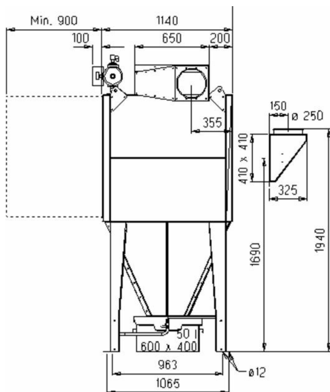
FMK(Z)25-2E Bin All dimensions in mm. If 50 liter bin with rollers, add 90 mm. * 65 mm to be included at top mounted fan
