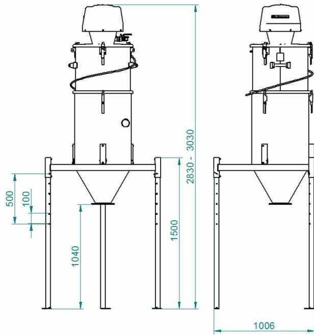
Dimensions with 1 500 mm legs
