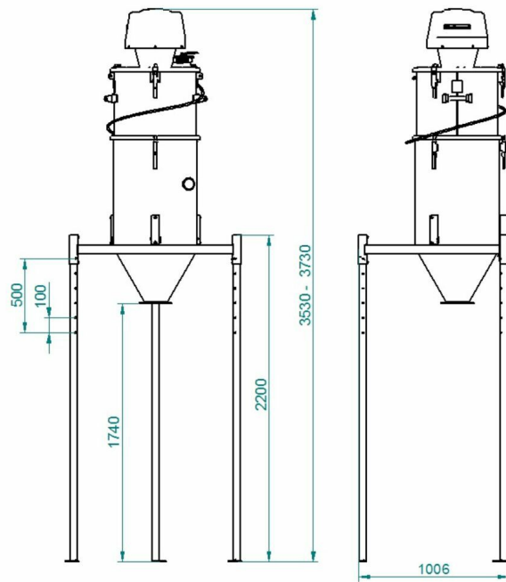
Dimensions with 2200 mm legs
