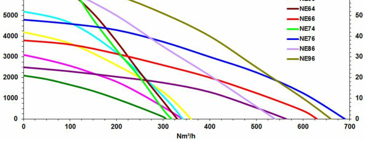
Air Powered ejectors All performance data are based on 7 bar supply pressure
