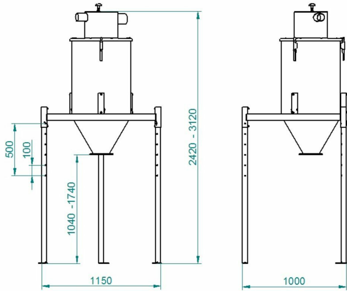
Dimensions pre-separation part
