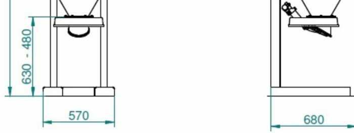
Dimensions - Filter part
