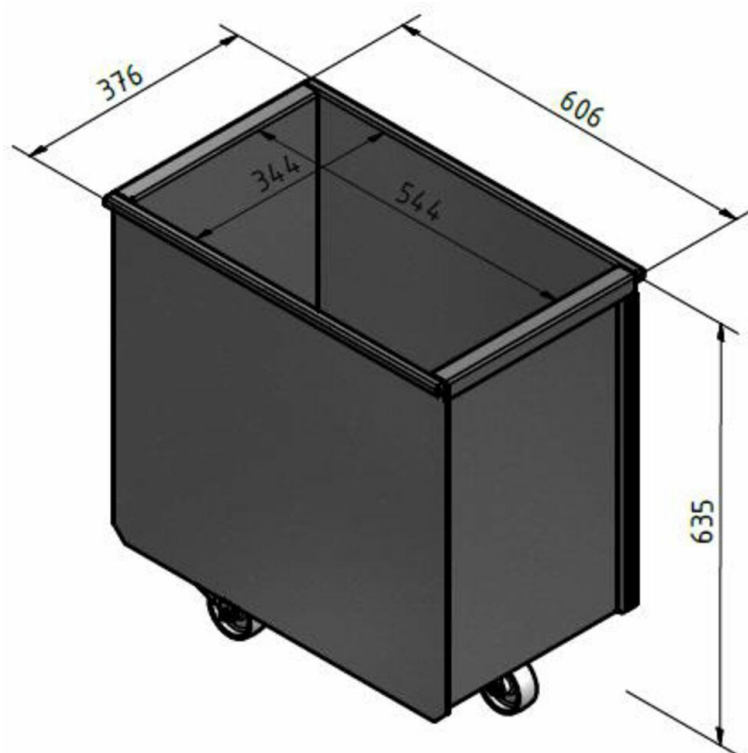
100 Liter Discharge bin with wheels
