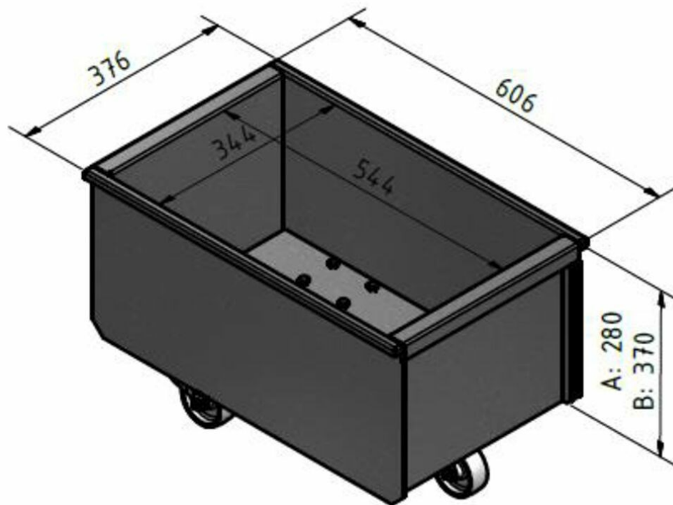
50 Liter Discharge bin without wheels (A) Discharge bin with wheels (B)
