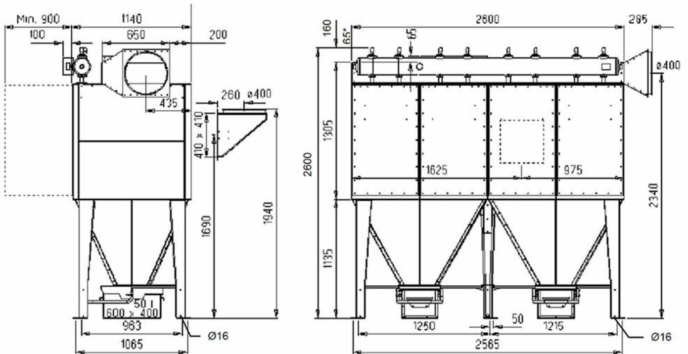
MK(Z)25-8E Bin All dimensions in mm. If 50 liter bin with rollers, add 90 mm. * 65 mm to be included at top mounted fan
