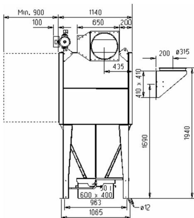
FMK(Z)25-6E Bin All dimensions in mm. If 50 liter bin with rollers, add 90 mm. * 65 mm to be included at top mounted fan
