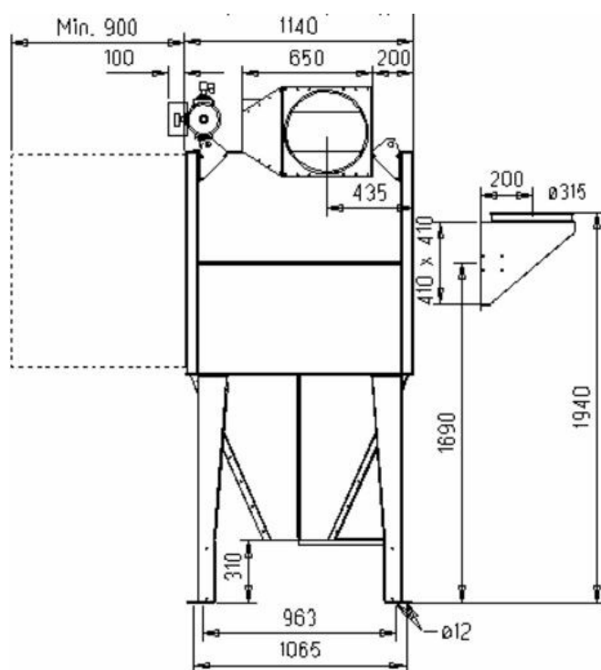
FMK(Z)25-6E Flange All dimensions in mm. * 65 mm to be included at top mounted fan.
