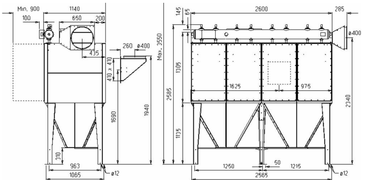
MK(Z)25-8E Flange All dimensions in mm. * 65 mm to be included at top mounted fan.
