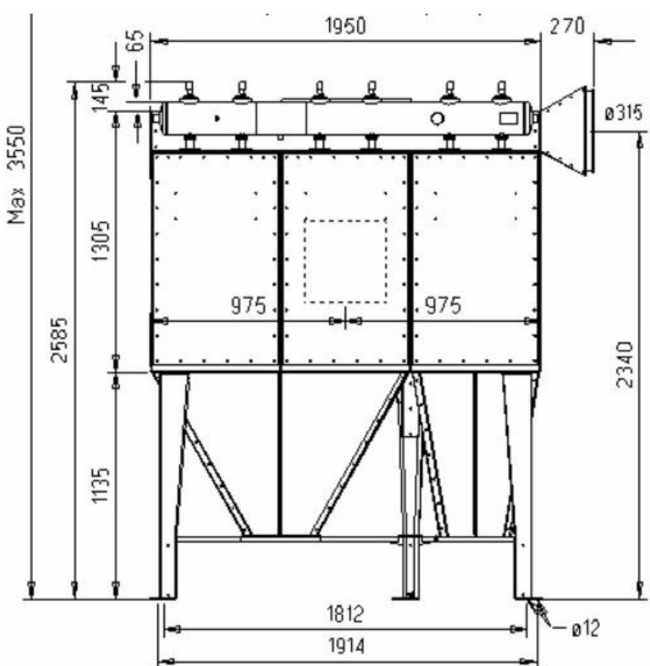
FMK(Z)25-6E Flange All dimensions in mm. * 65 mm to be included at top mounted fan.
