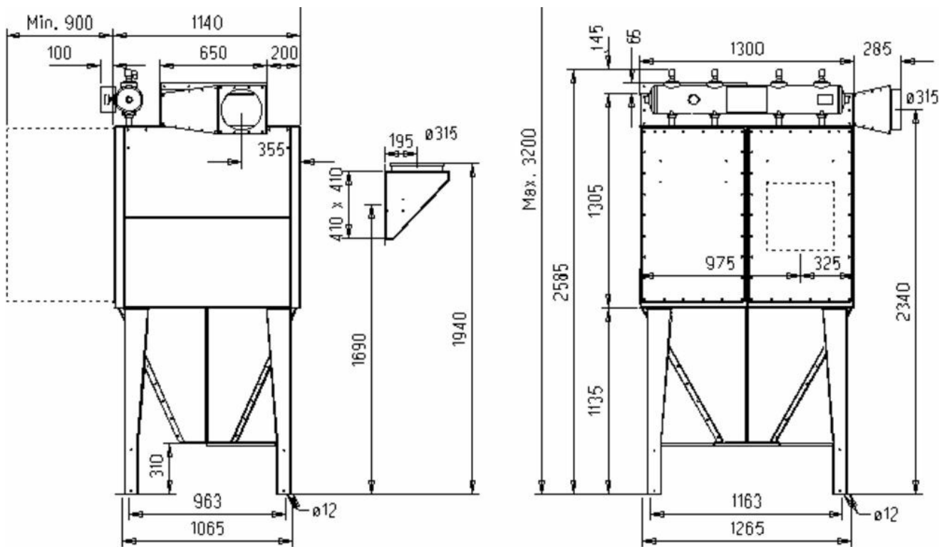
MK(Z)25-4E Flange All dimensions in mm. * 65 mm to be included at top mounted fan.
