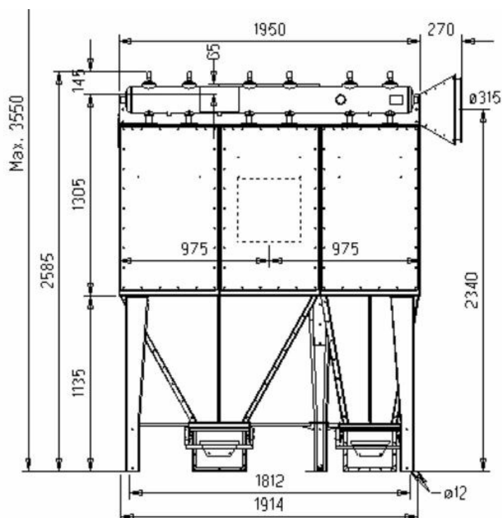
FMK(Z)25-6E Bin All dimensions in mm. If 50 liter bin with rollers, add 90 mm. * 65 mm to be included at top mounted fan
