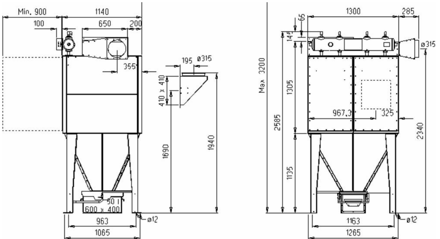
FMK(Z)25-4E Bin All dimensions in mm. If 50 liter bin with rollers, add 90 mm. * 65 mm to be included at top mounted fan
