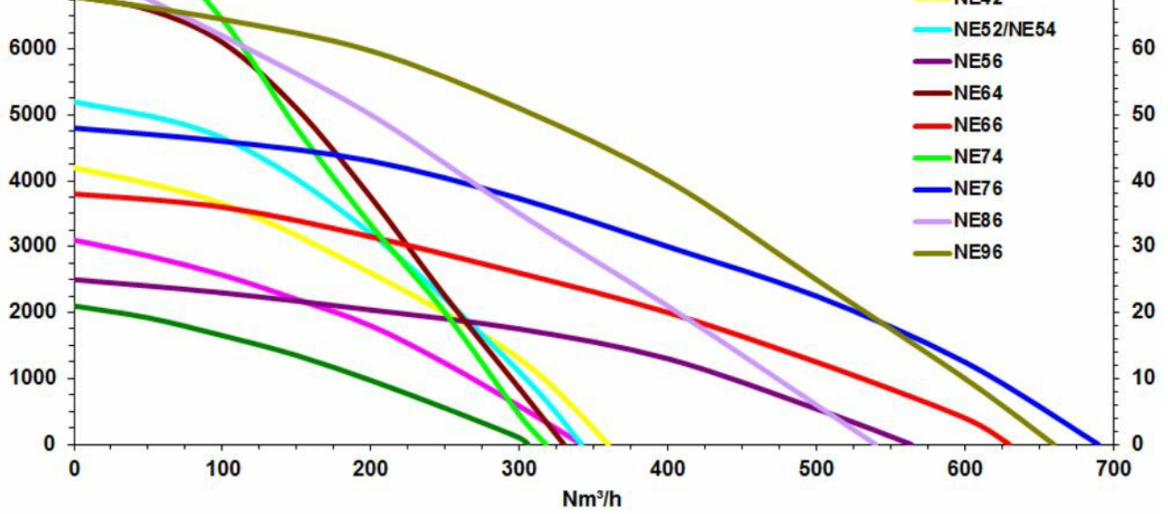
Air Powered ejectors All performance data are based on 7 bar supply pressure
