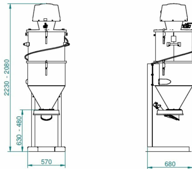
Dimensions - Filter part
