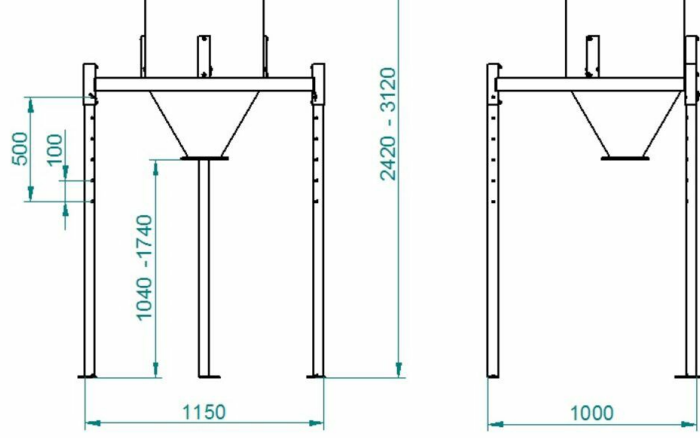
Dimensions pre-separation part
