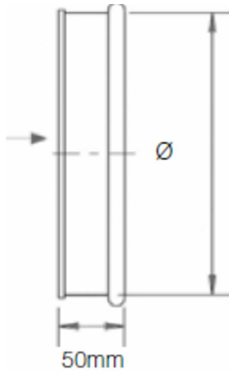
QF End Cap Dimensions, 22012-XXX
