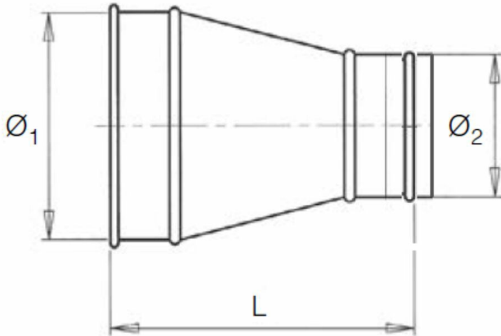
QF Cone for hose connection dimensions
