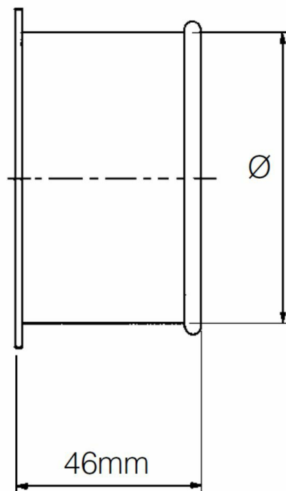
QF Tabular rivet adapter dimensions
