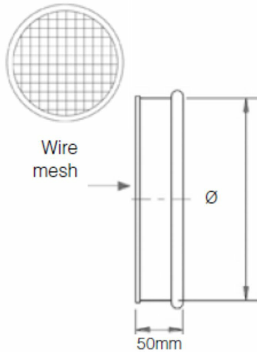
QF Mesh End Cap Dimensions
