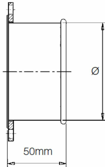
QF Flanged adapter dimensions
