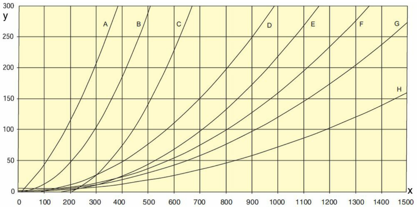
Y = Pressure drop Pa/m X = Airflow m 3 /h A = Ø75 mm (3") on reel B = Ø75 mm (3") straight C = Ø100 mm (4") on reel D = Ø125 mm (5") on reel E = Ø100 mm (4") straight F = Ø150 mm (6") on reel G = Ø125 mm (5") straight H = Ø150 mm (6") straight
