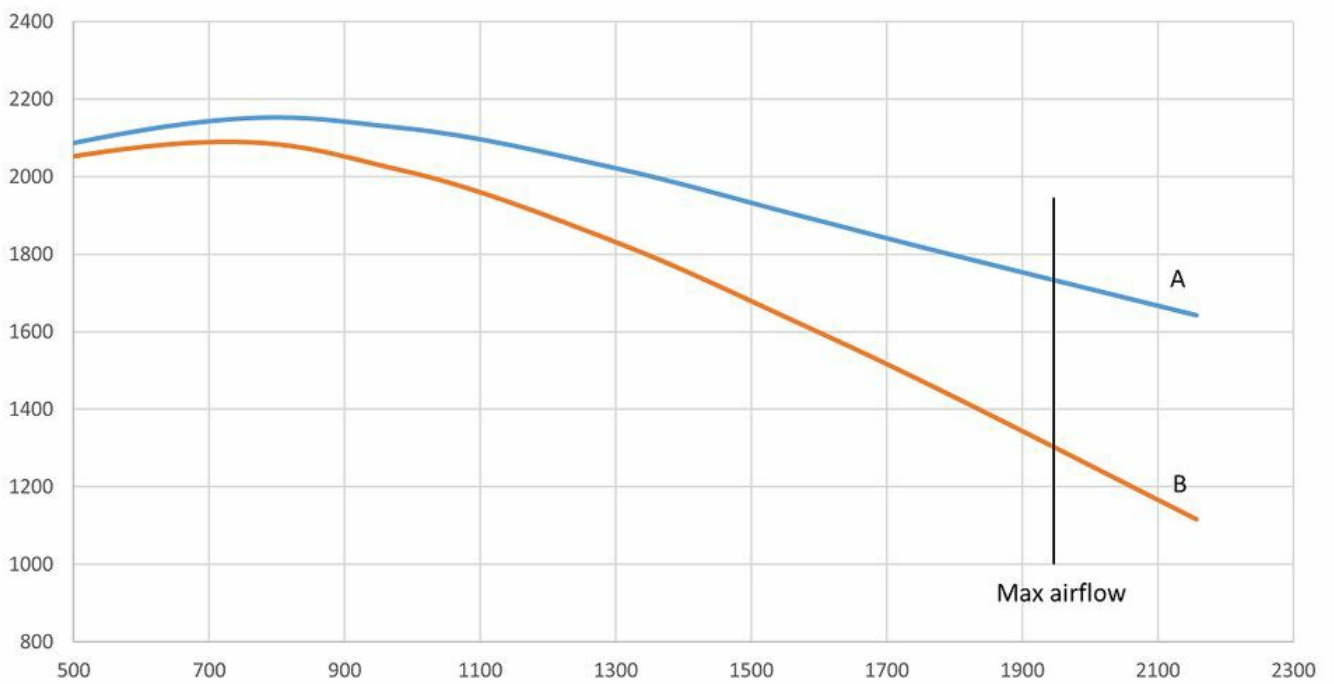
A: Total Pressure B: Static Pressure X-Axis: m³/h Y-Axis: Pa
